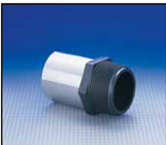
Part # P20 Fitting Material Polypropylene Stainless Steel Collar
